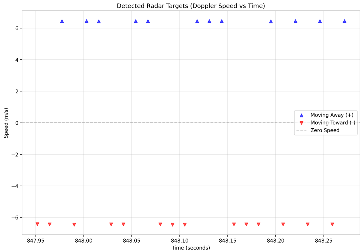
Figure 9. Python Code Speed Data Plot (1024 Hz Tuning Fork or 6.3 m/s)
