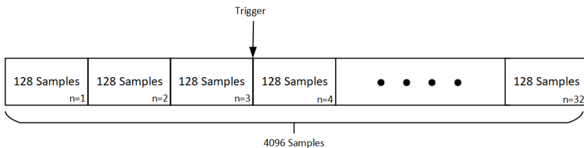
Figure 2. Rolling Buffer Architecture
