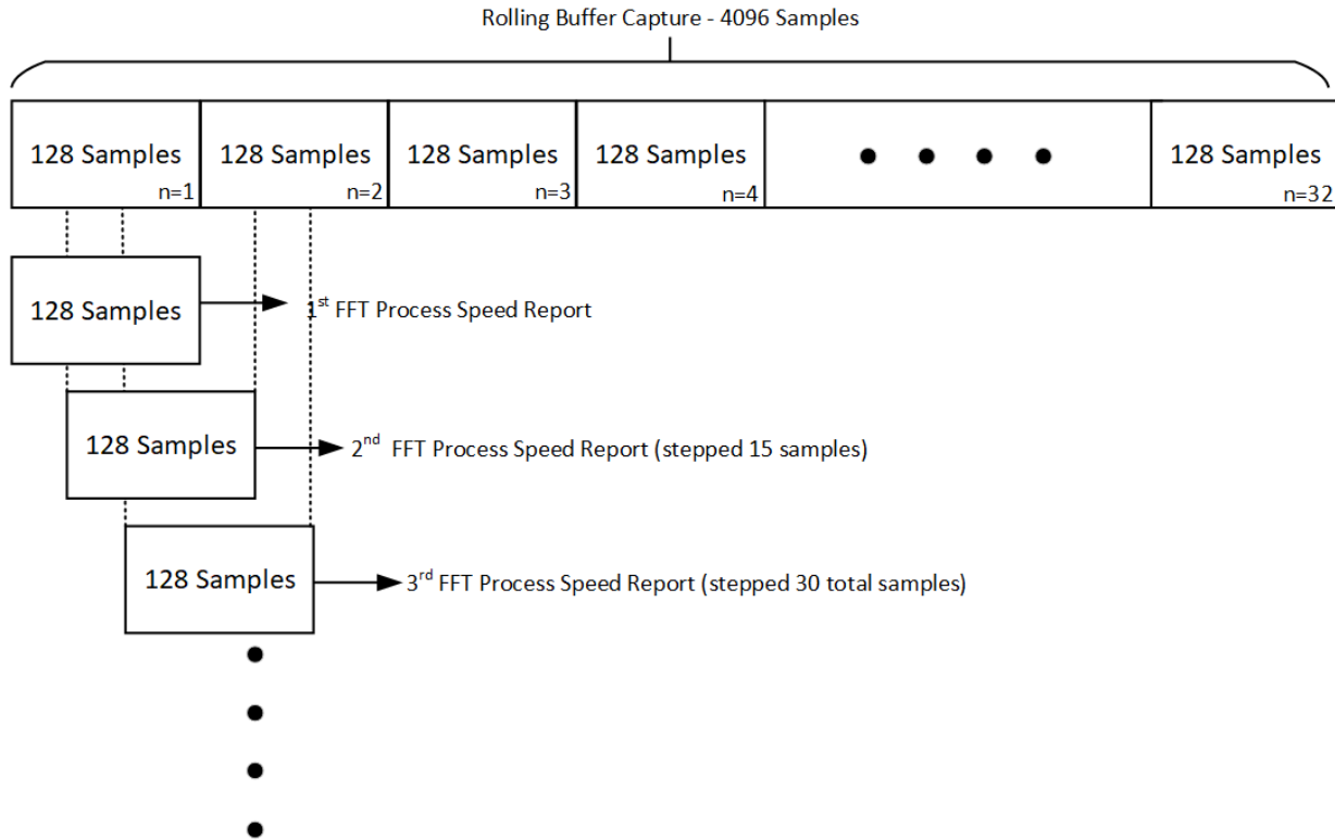
Figure 6. Stepped Samples FFT Processing
