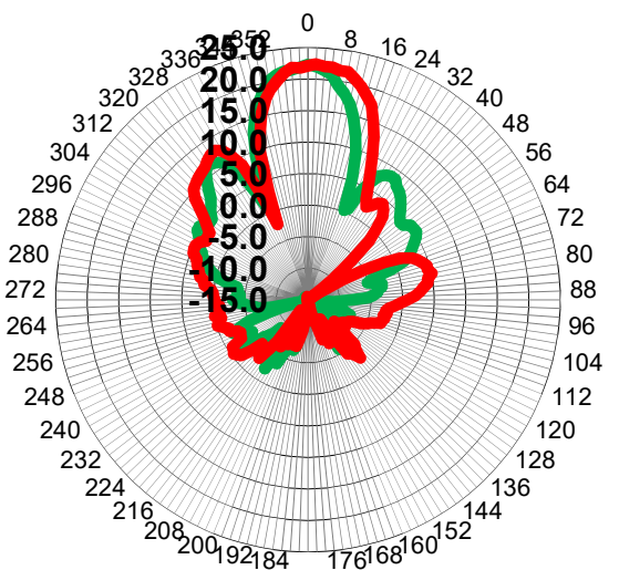
Antenna Pattern
