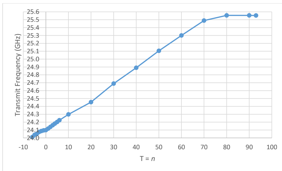
Figure 6. Frequency Setting T Values
